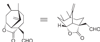
Figure 1. Structure of (+)-upial ( 1 ).
